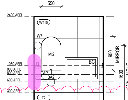
VILLAGE AMENITIES - ACC WC - 3
