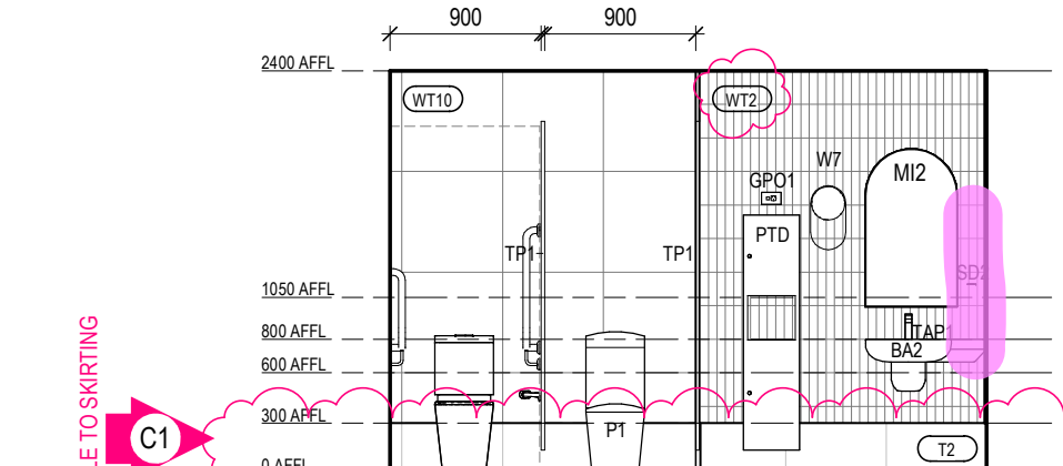
VILLAGE AMENITIES - FEMALE WC - 1
