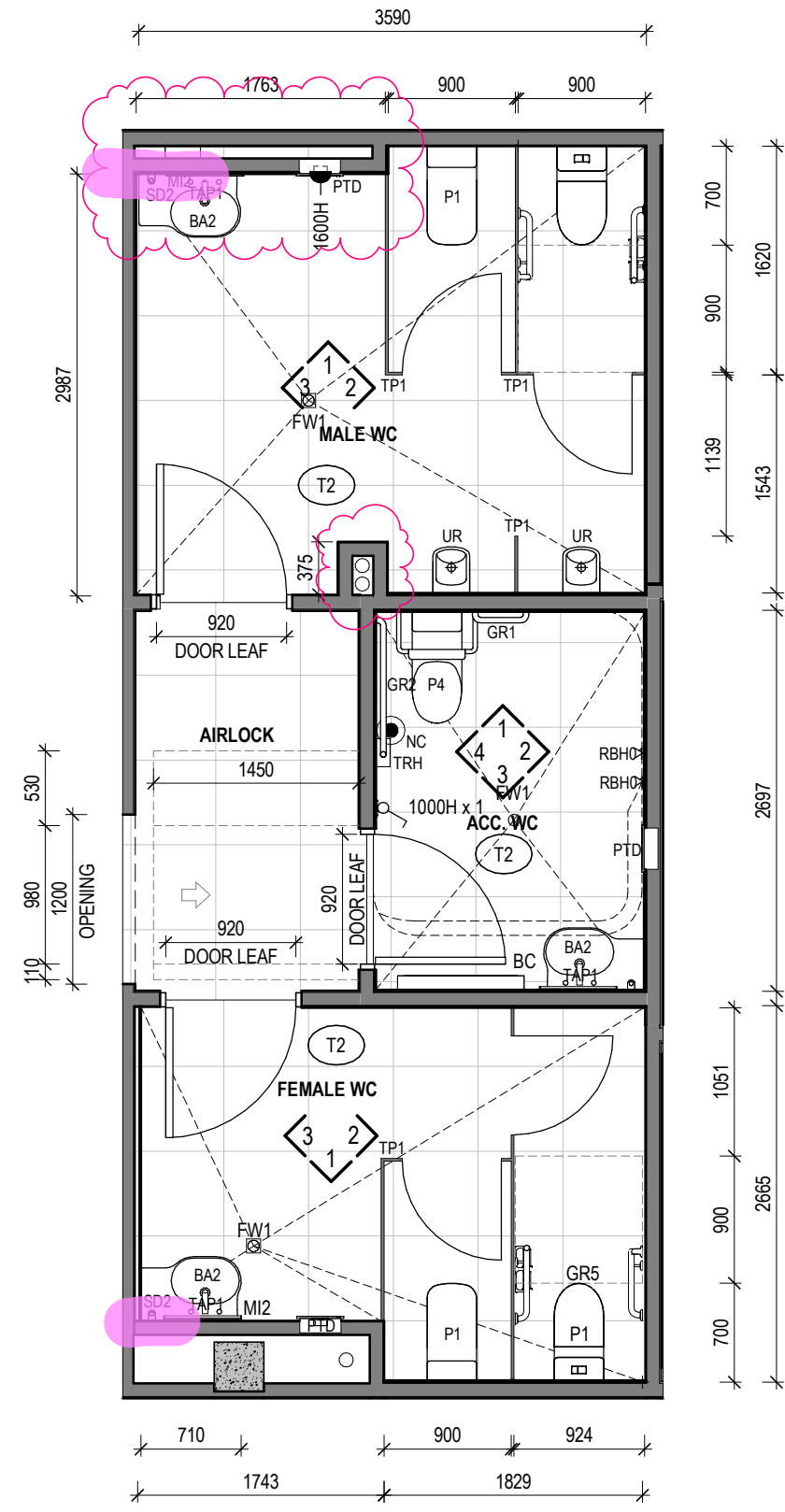
1 VILLAGE LIFESTYLE - AMENITIES Scale 1: 50
