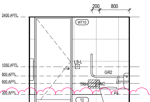
VILLAGE AMENITIES - ACC WC - 4
