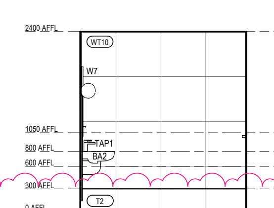
VILLAGE AMENITIES - FEMALE WC - 3
