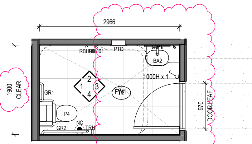
4 RACF AMENITIES - ACCESSIBLE WC 02 Scale 1: 50
