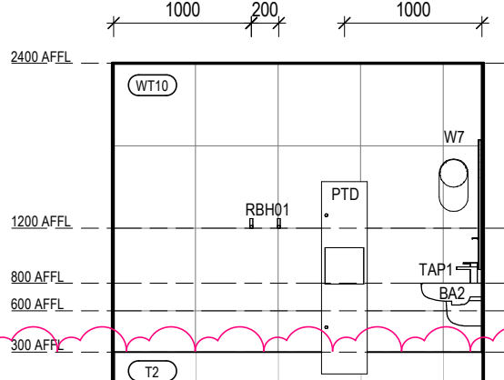
VILLAGE AMENITIES - ACC WC - 2
