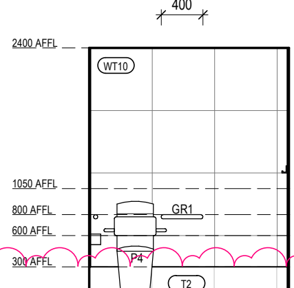
VILLAGE AMENITIES - ACC WC - 1
