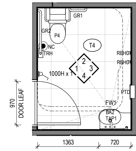
3 RACF AMENITIES - ACCESSIBLE WC 01 Scale 1: 50
